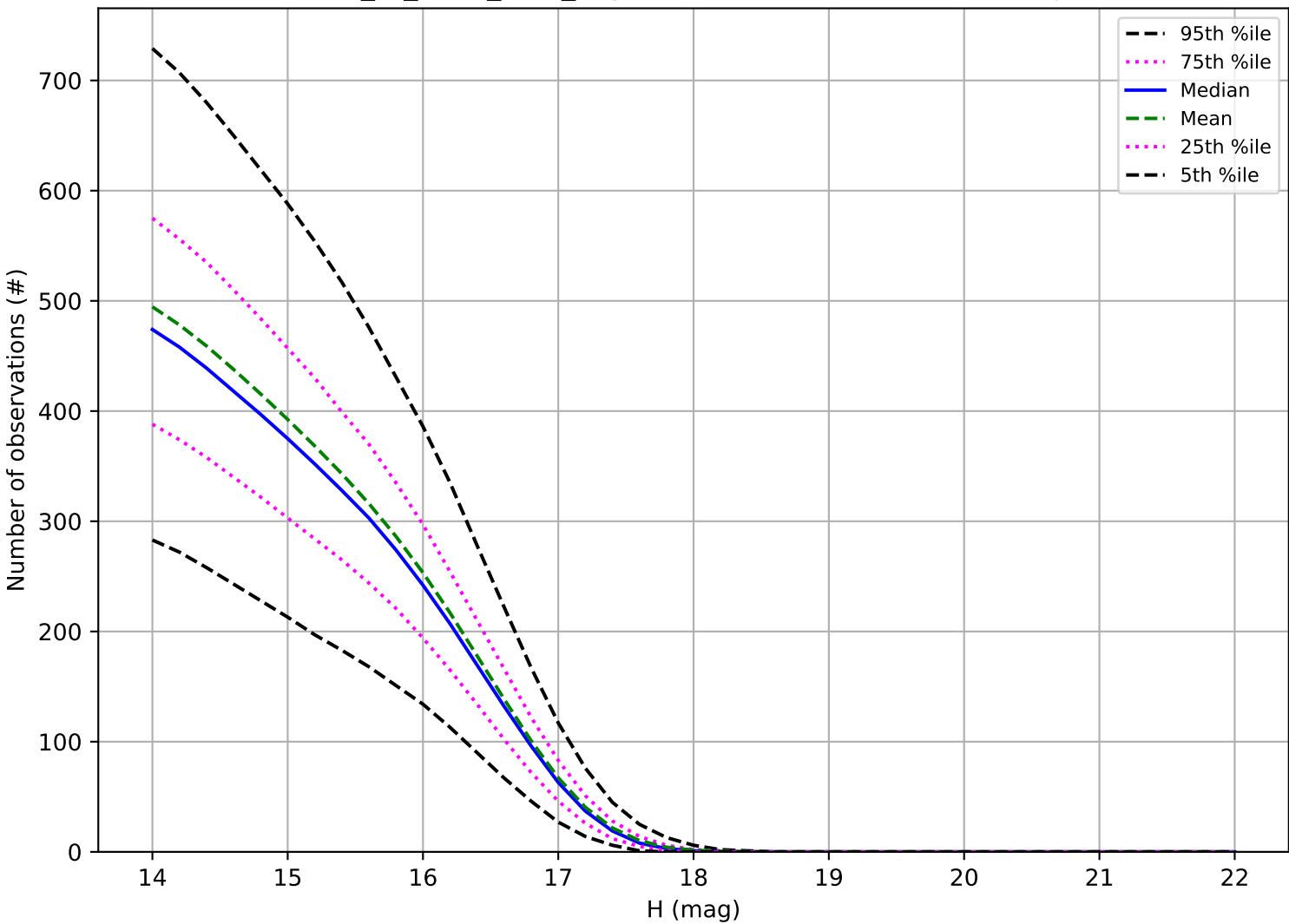
extra_ss_neo2_v3.4_10yrs: Number of observations Trojan
