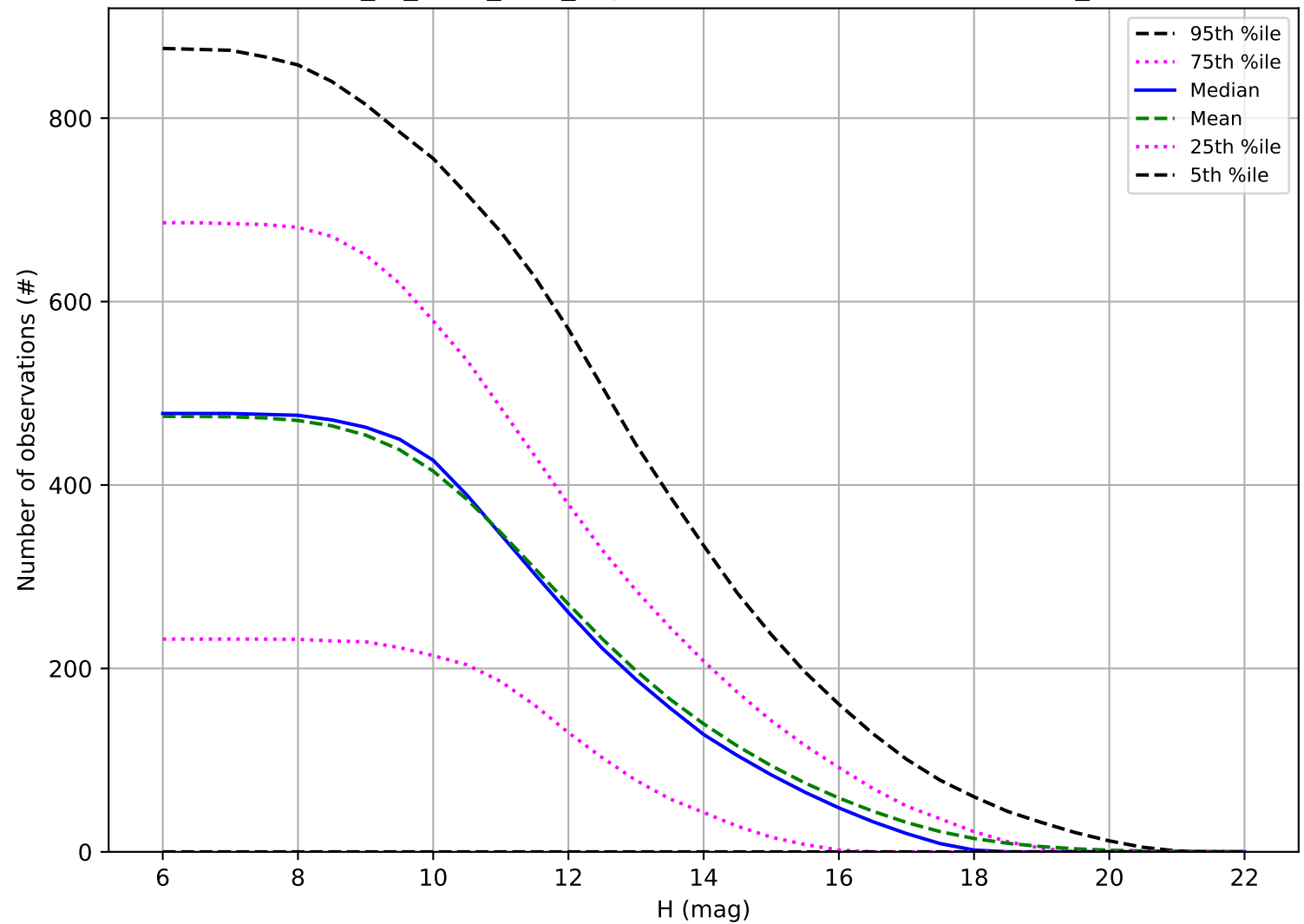
extra_ss_neo2_v3.4_10yrs: Number of observations OCC_r5
