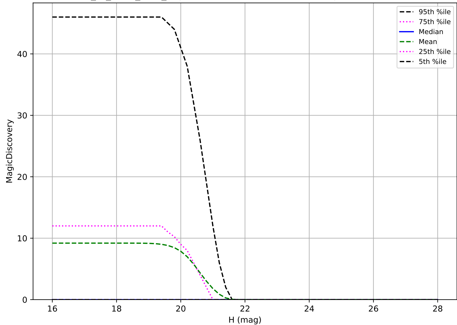
extra_ss_neo2_v3.4_10yrs: Vatira 6 detections in 60 nights detection loss
