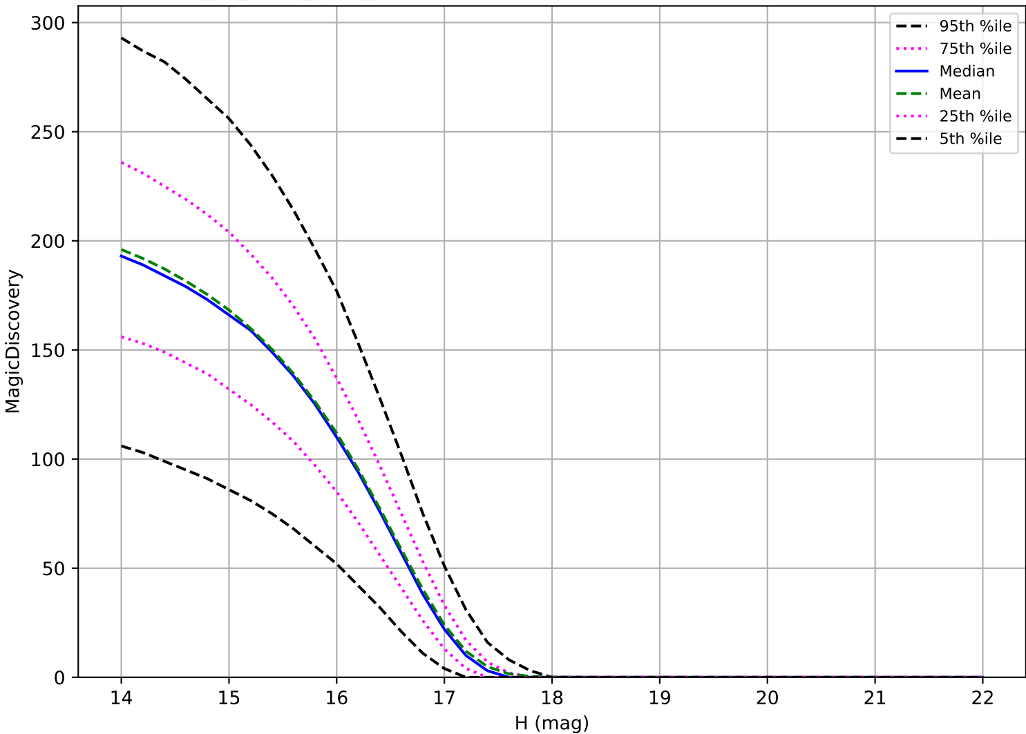
extra_ss_neo2_v3.4_10yrs: Trojan 6 detections in 60 nights detection loss
