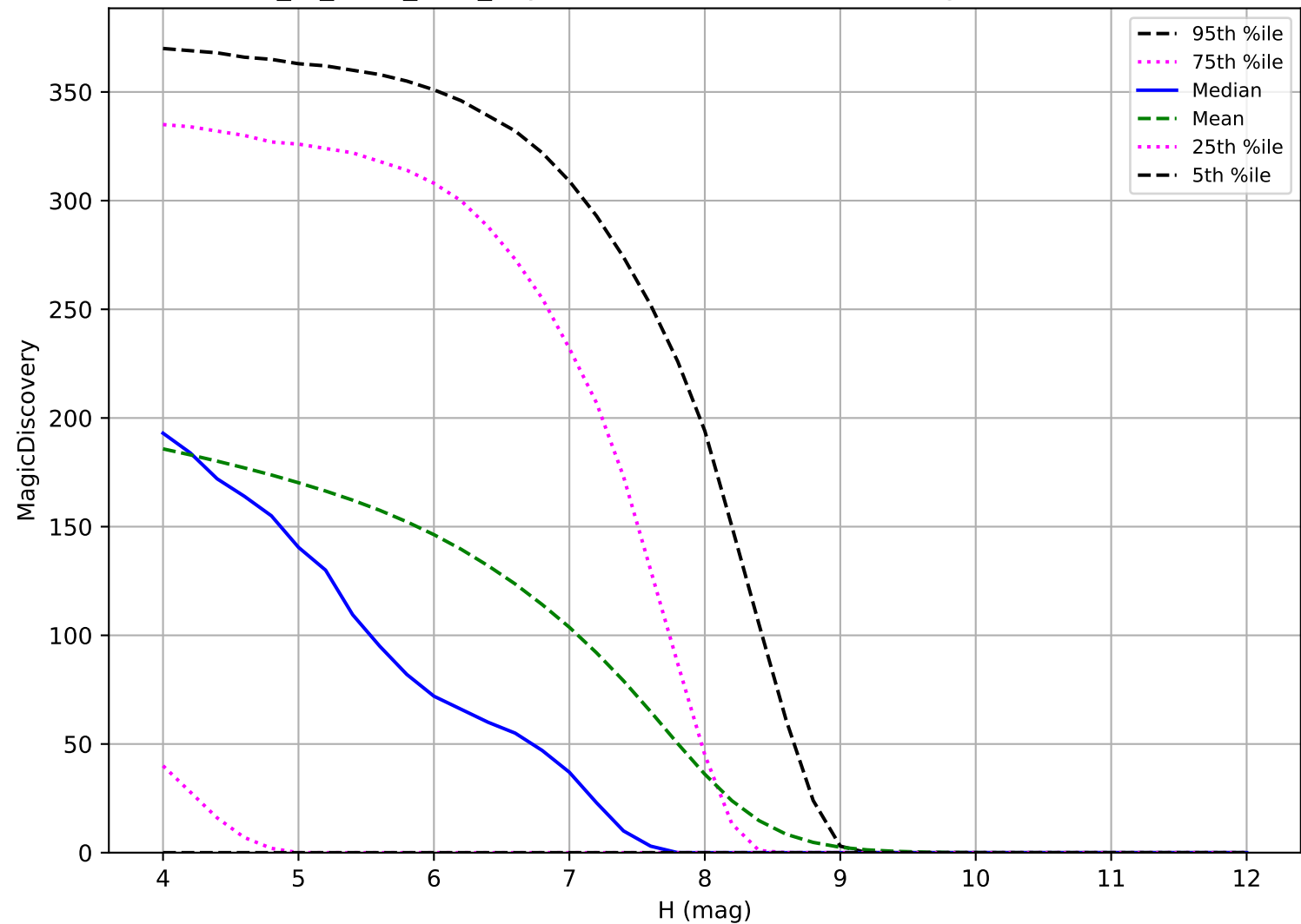
extra_ss_neo2_v3.4_10yrs: TNO 6 detections in 60 nights detection loss
