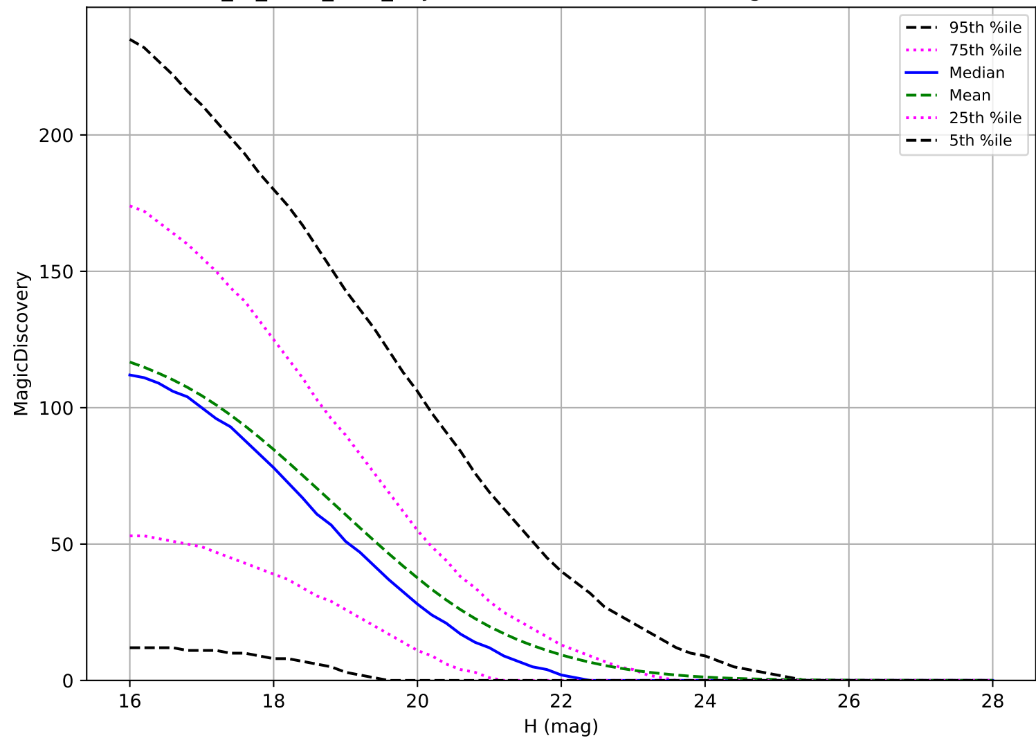
extra_ss_neo2_v3.4_10yrs: PHA 6 detections in 60 nights detection loss
