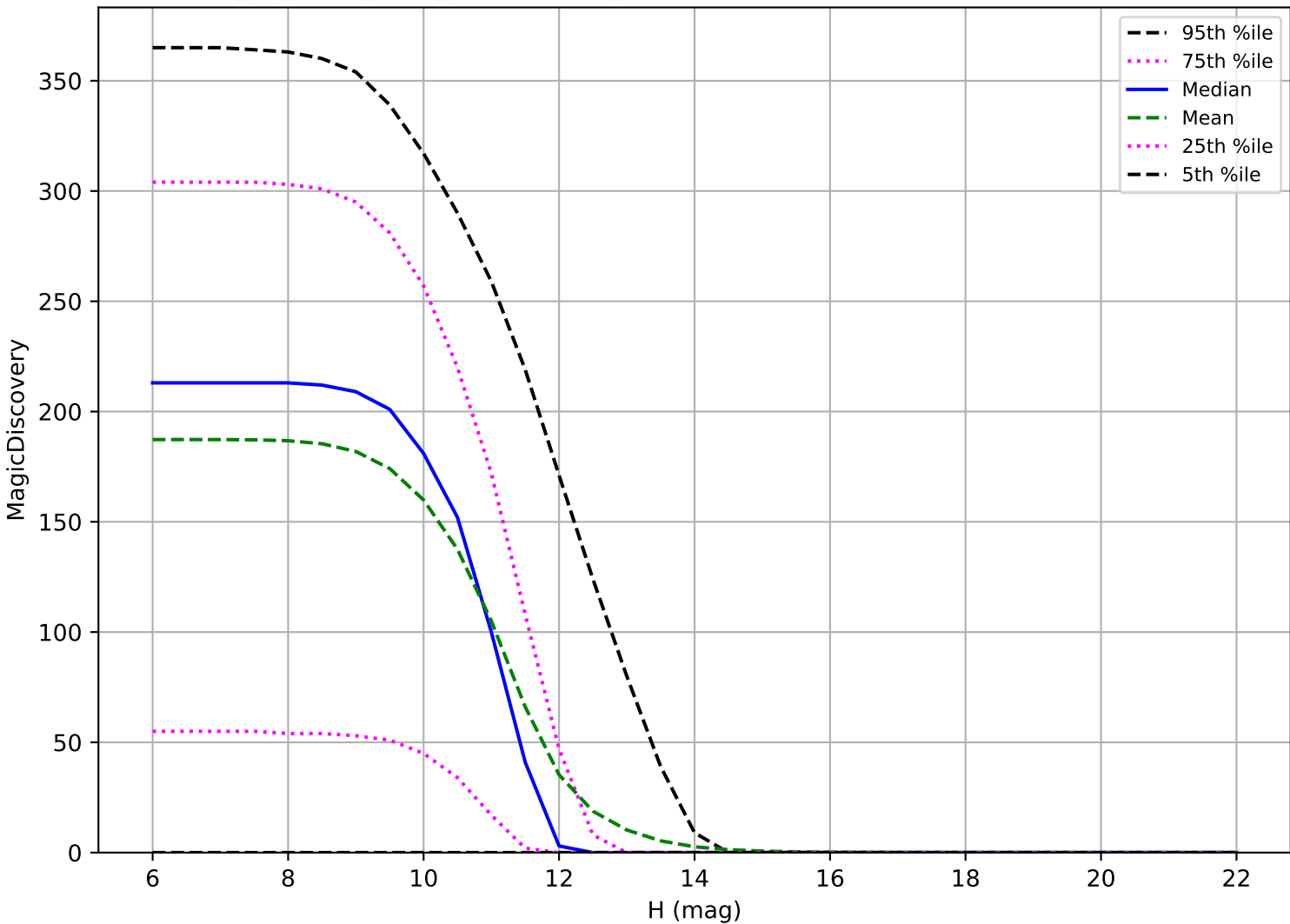
extra_ss_neo2_v3.4_10yrs: OCC_r20 6 detections in 60 nights detection loss
