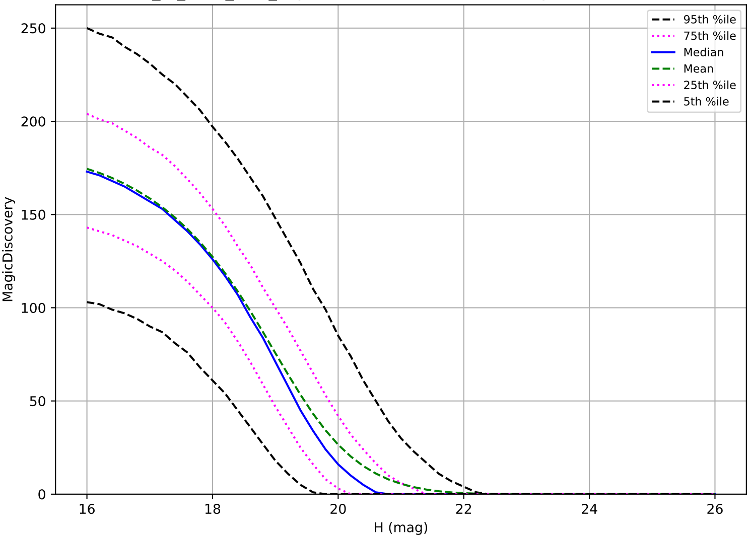
extra_ss_neo2_v3.4_10yrs: MBA 6 detections in 60 nights detection loss
