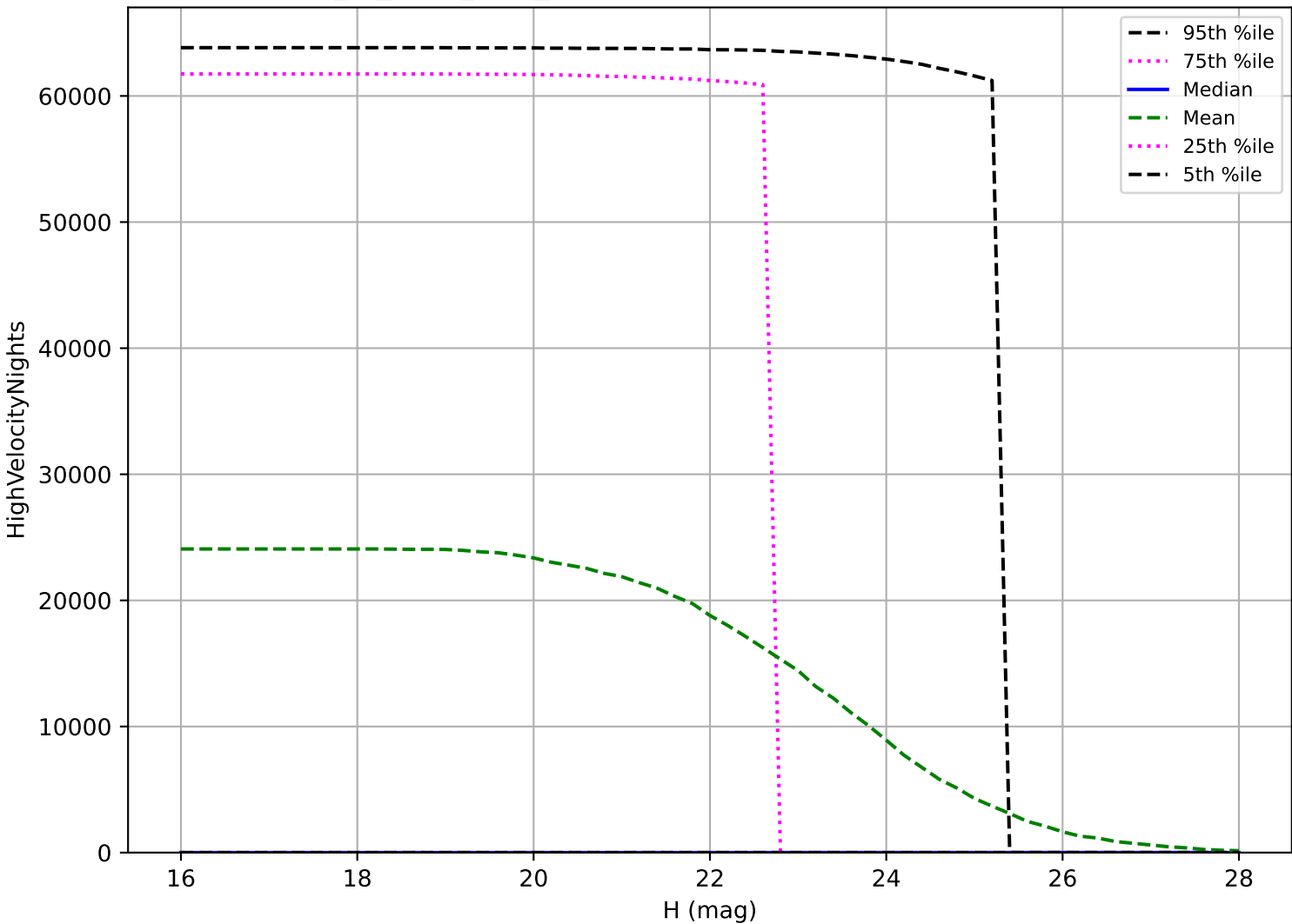
extra_ss_neo2_v3.4_10yrs: PHA High velocity pair detection loss
