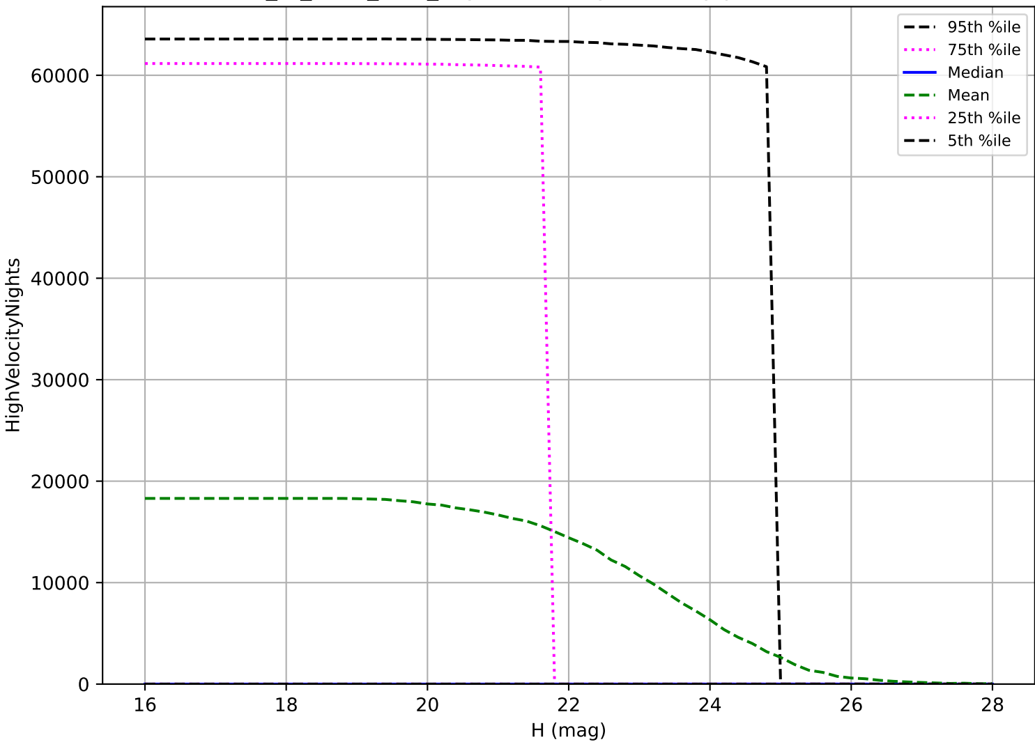
extra_ss_neo2_v3.4_10yrs: NEO High velocity pair detection loss
