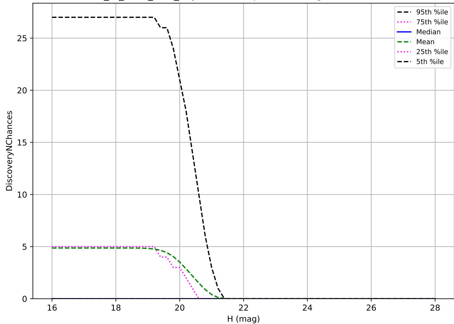
extra_ss_neo2_v3.4_10yrs: Vatira 3 pairs in 15 nights detection loss
