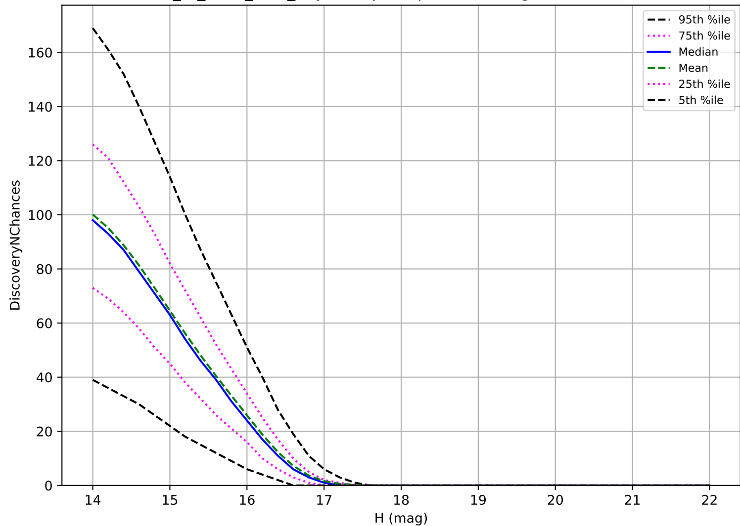
extra_ss_neo2_v3.4_10yrs: Trojan 3 pairs in 15 nights detection loss
