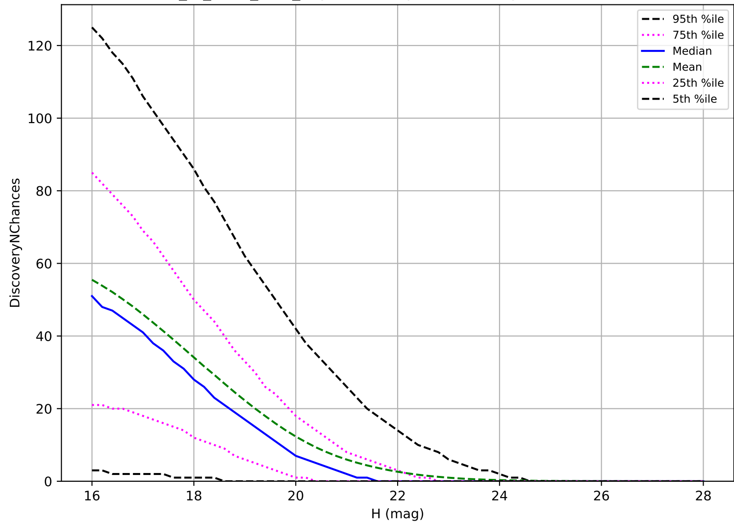
extra_ss_neo2_v3.4_10yrs: PHA 3 pairs in 15 nights detection loss
