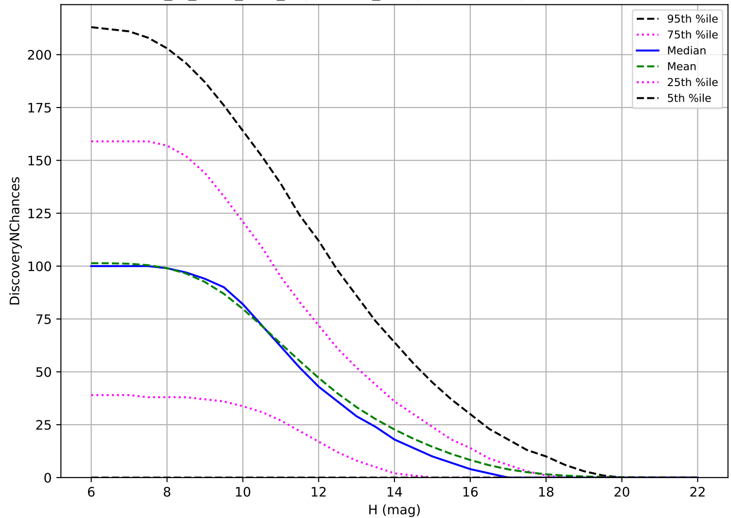
extra_ss_neo2_v3.4_10yrs: OCC_r5 3 pairs in 15 nights detection loss
