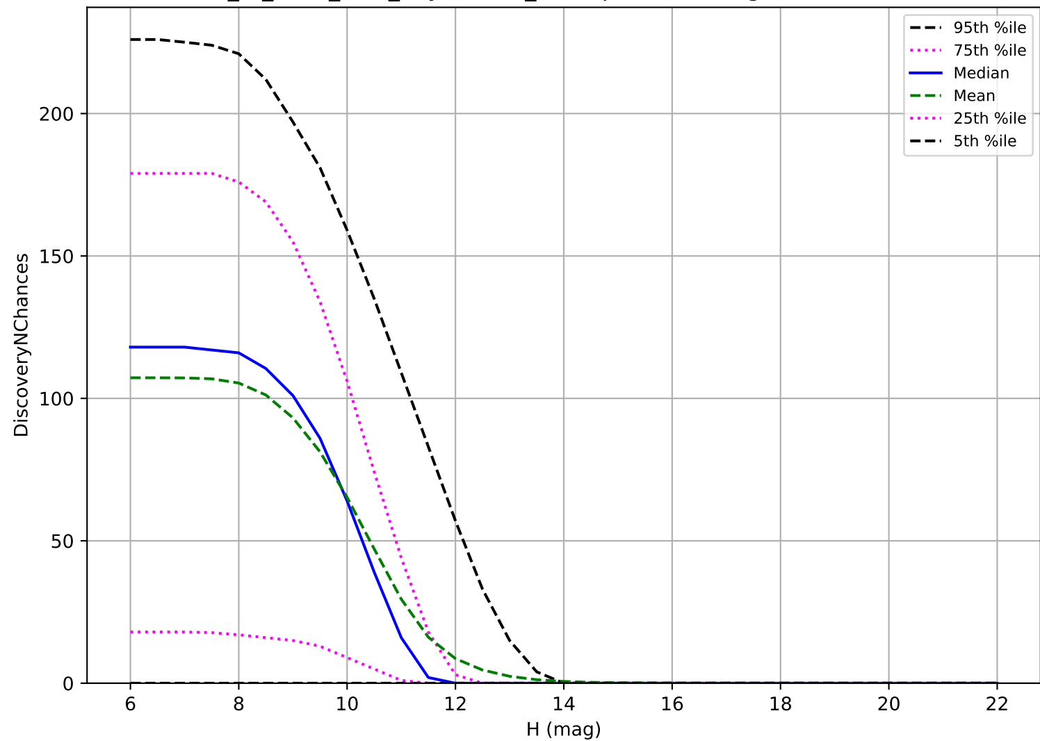
extra_ss_neo2_v3.4_10yrs: OCC_r20 3 pairs in 15 nights detection loss
