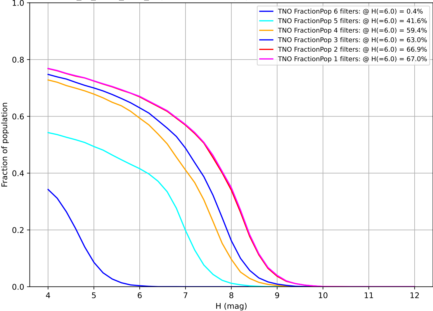
extra_ss_neo2_v3.4_10yrs: Fraction of population with colors in X filters TNO
