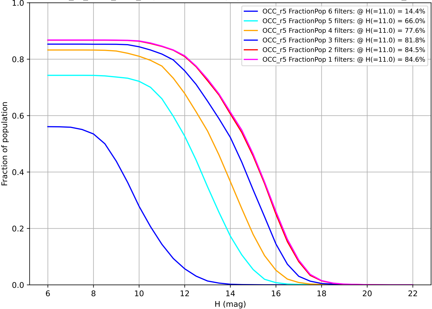
extra_ss_neo2_v3.4_10yrs: Fraction of population with colors in X filters OCC_r5
