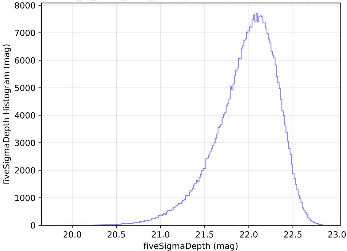
extra_ss_neo2_v3.4_10yrs y: fiveSigmaDepth Histogram
