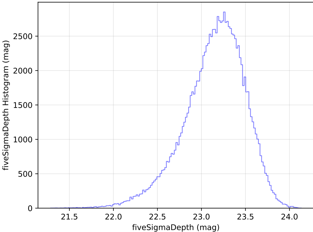
extra_ss_neo2_v3.4_10yrs u: fiveSigmaDepth Histogram
