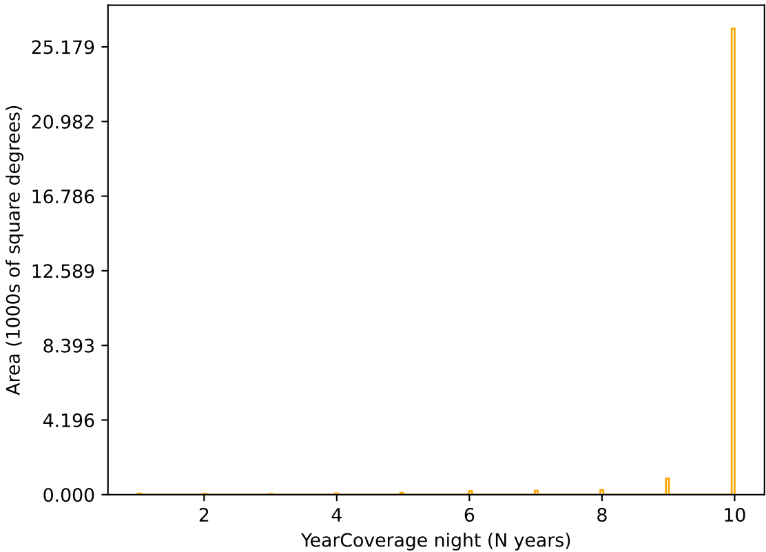
extra_ss_neo2_v3.4_10yrs r band: YearCoverage night
