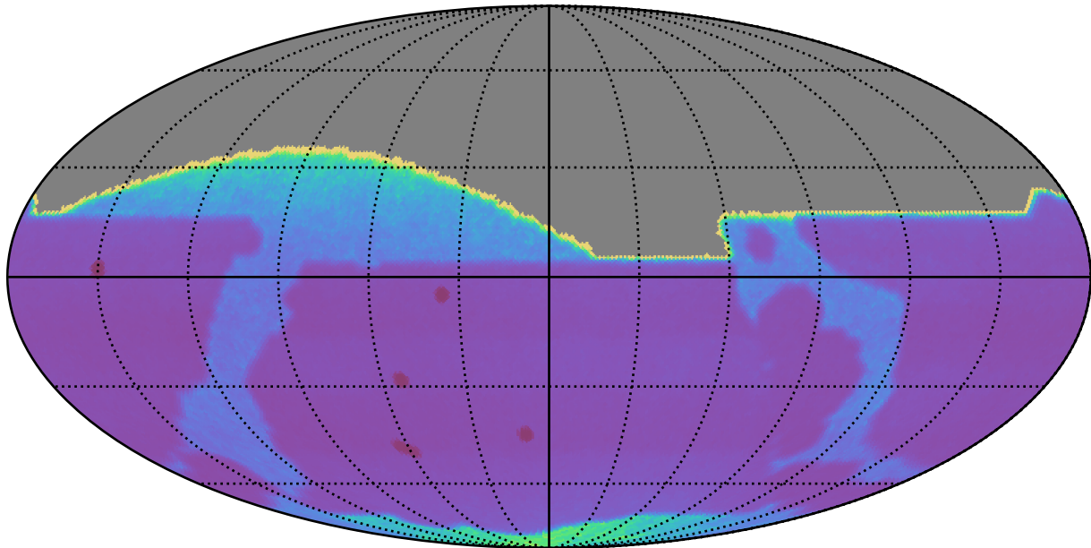
extra_ss_neo2_v3.4_10yrs : Proper Motion Uncert @ 20.5
