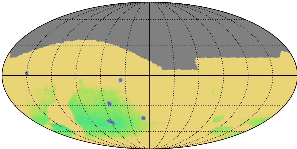
extra_ss_neo2_v3.4_10yrs : Parallax Uncert @ 22.4
