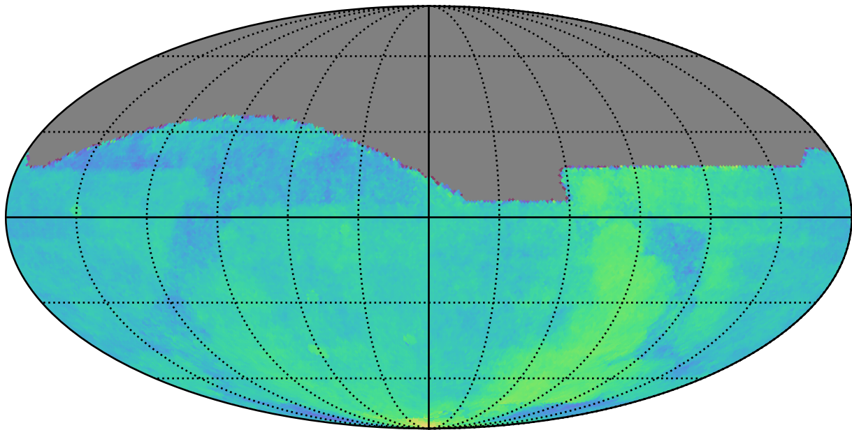
extra_ss_neo2_v3.4_10yrs : Parallax Coverage @ 22.4
