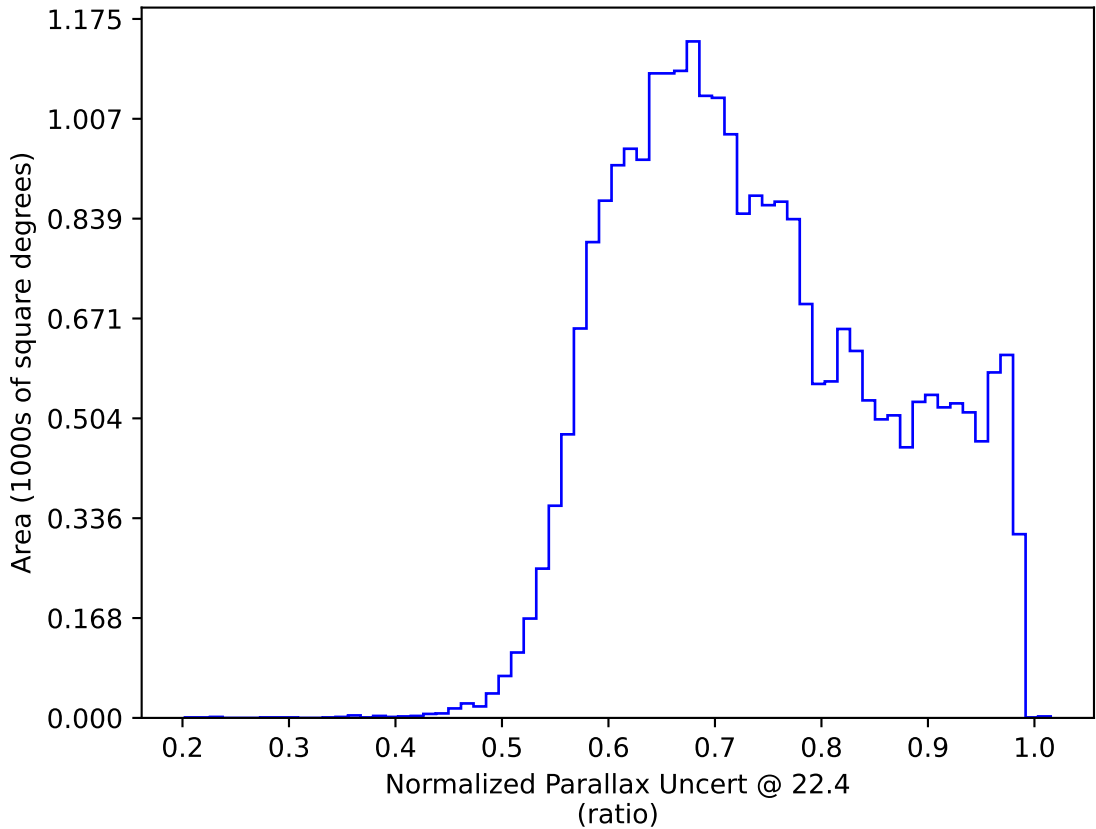
extra_ss_neo2_v3.4_10yrs : Normalized Parallax Uncert @ 22.4
