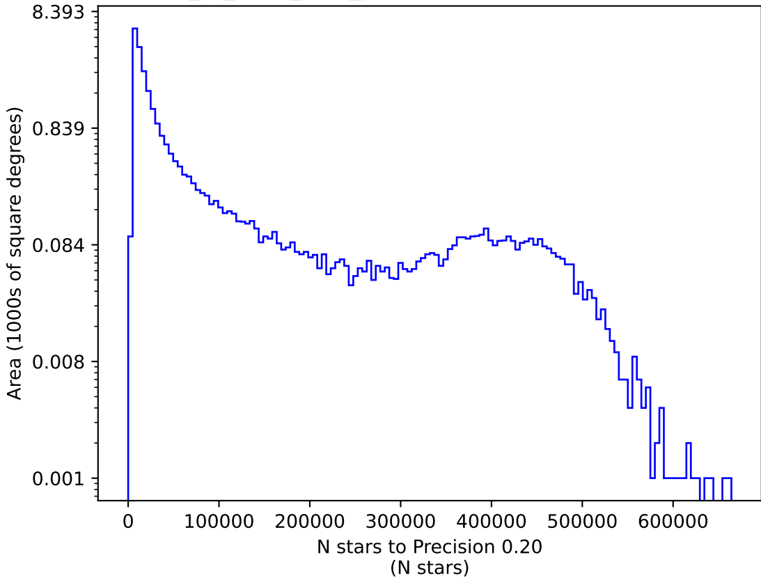
extra_ss_neo2_v3.4_10yrs z: N stars to Precision 0.20
