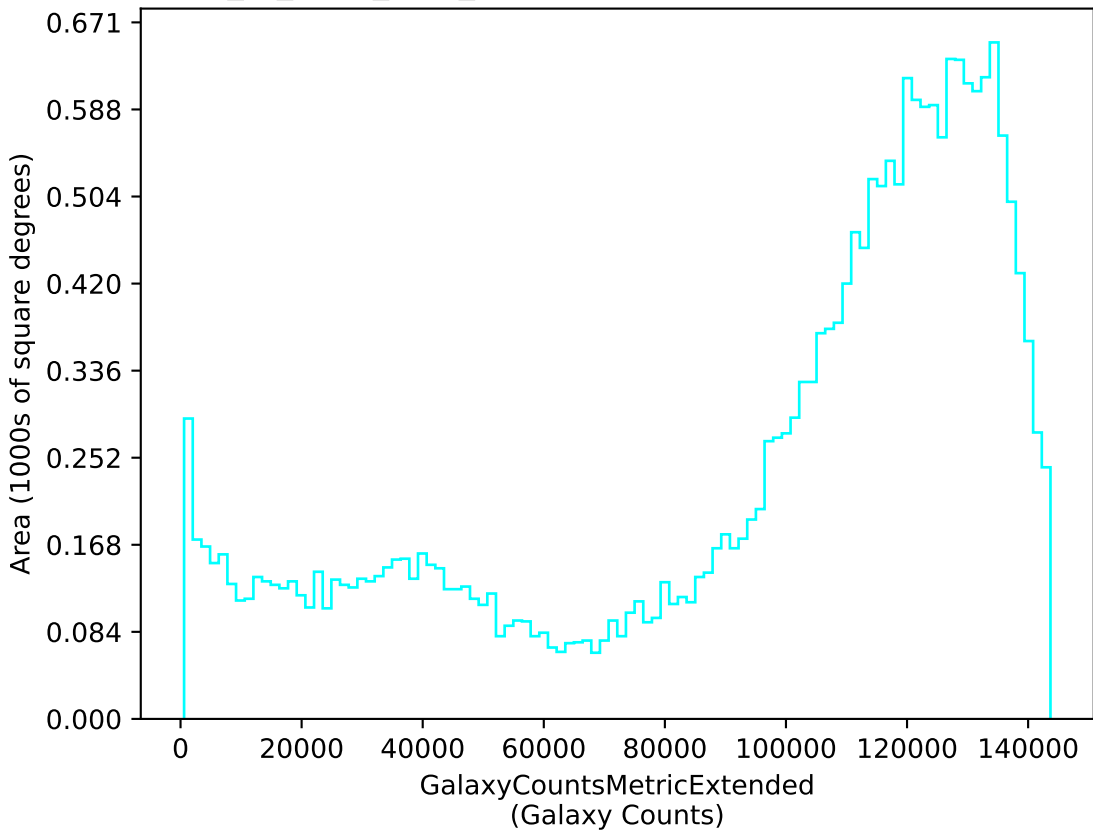
extra_ss_neo2_v3.4_10yrs u: GalaxyCountsMetricExtended
