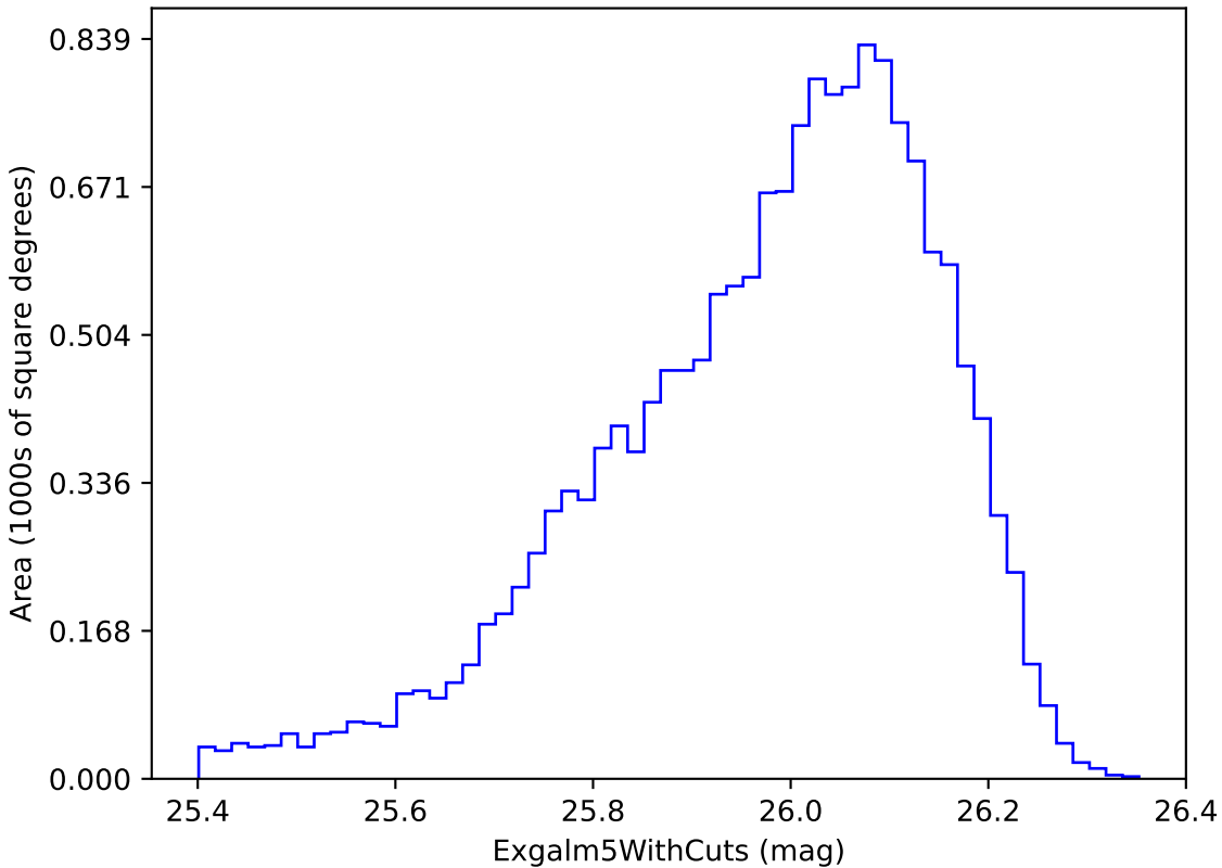
extra_ss_neo2_v3.4_10yrs i band non-DD year 4: Exgalml5WithCuts
