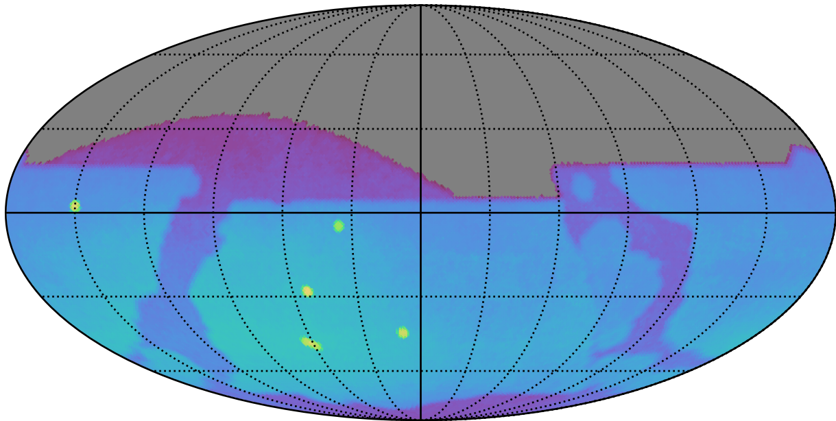
extra_ss_neo2_v3.4_10yrs : Brown Dwarf, L7
