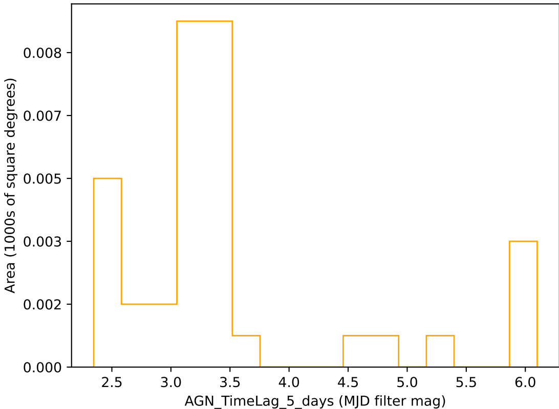
extra_ss_neo2_v3.4_10yrs r band: AGN_TimeLag_5_days
