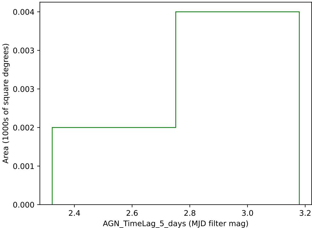
extra_ss_neo2_v3.4_10yrs g band: AGN_TimeLag_5_days
