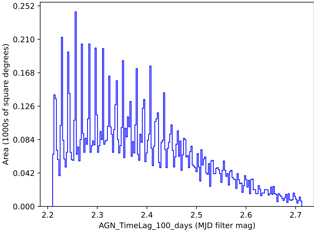
extra_ss_neo2_v3.4_10yrs y band: AGN_TimeLag_100_days
