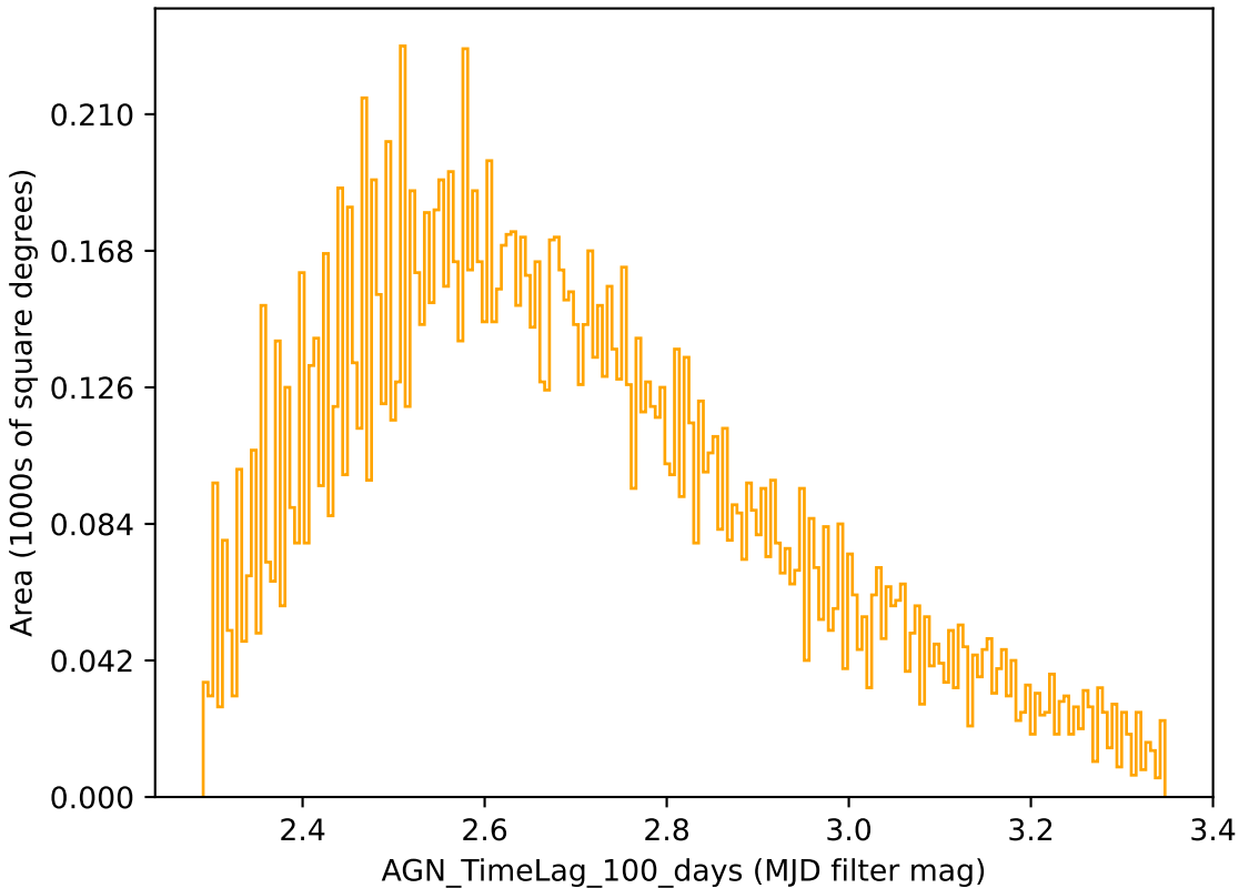
extra_ss_neo2_v3.4_10yrs r band: AGN_TimeLag_100_days
