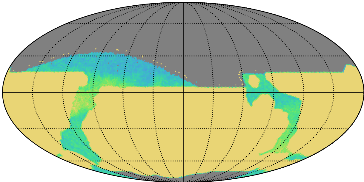
extra_ss_neo2_v3.4_10yrs all bands: AGN_TimeLag_100_days
