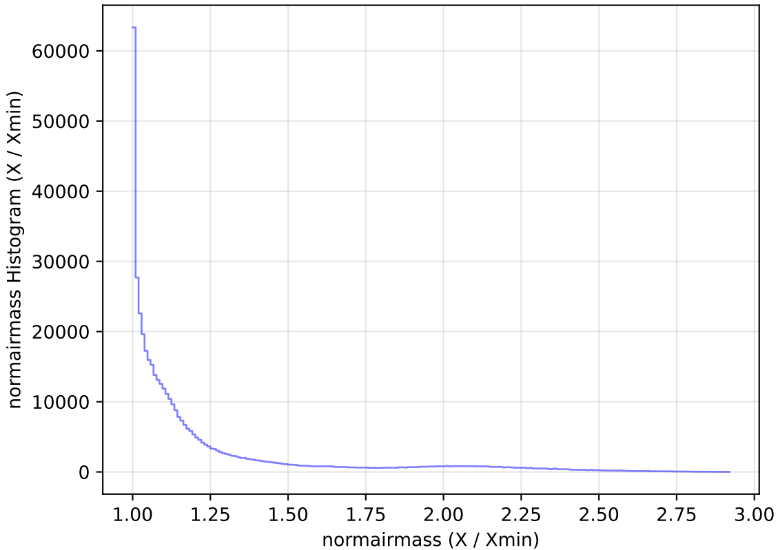
extra_ss_neo2_v3.4_10yrs WFD z band: normairmass Histogram
