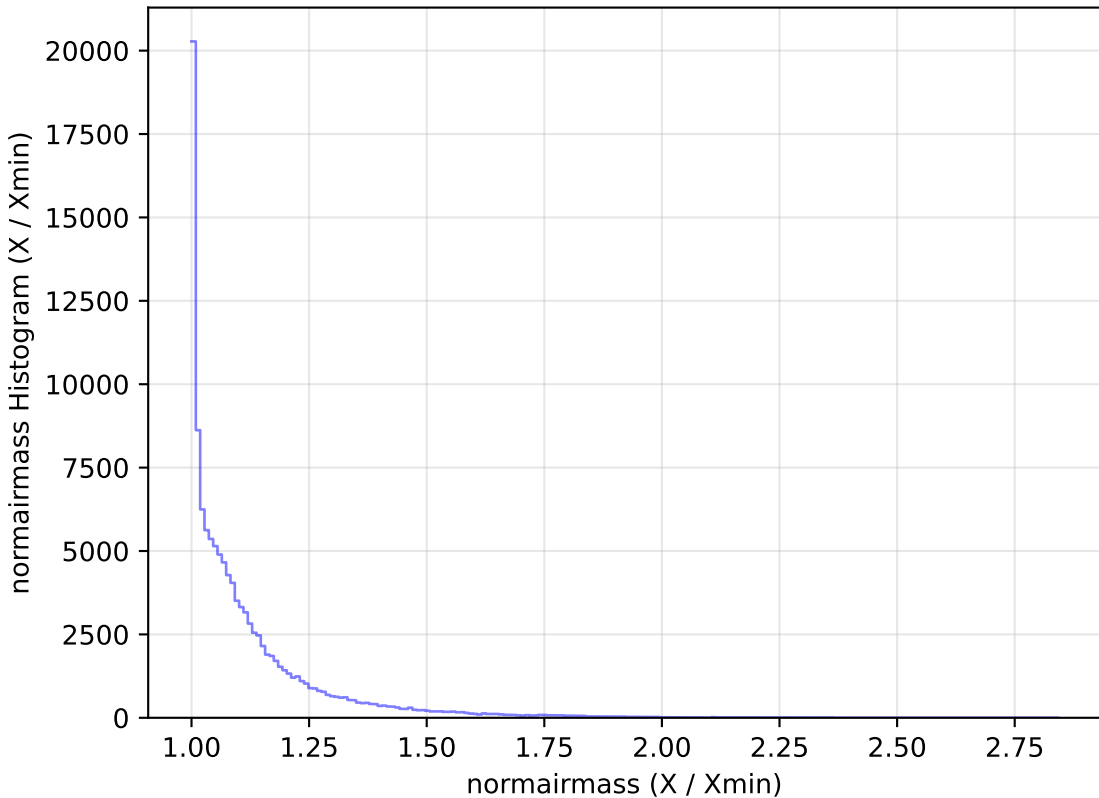
extra_ss_neo2_v3.4_10yrs WFD u band: normairmass Histogram
