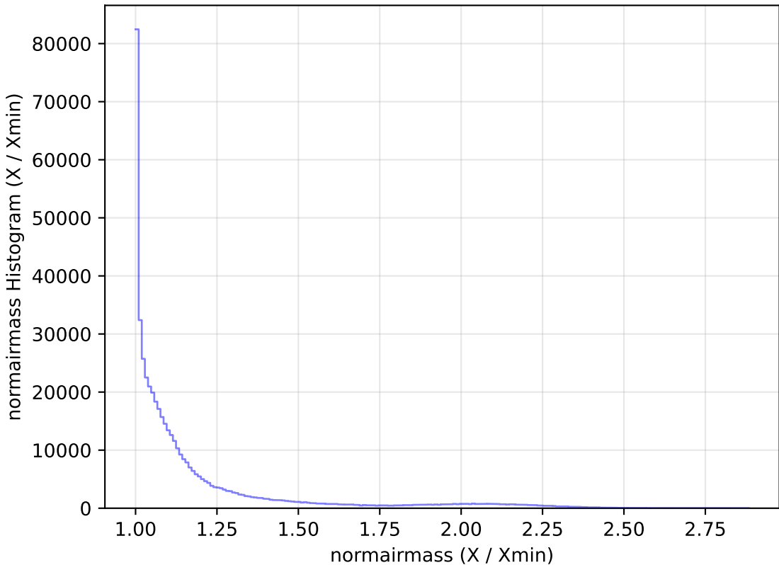
extra_ss_neo2_v3.4_10yrs WFD r band: normairmass Histogram
