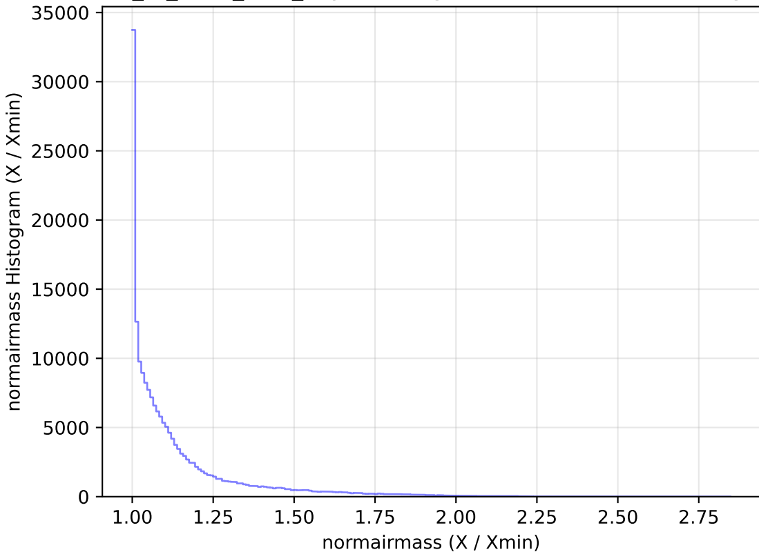
extra_ss_neo2_v3.4_10yrs WFD g band: normairmass Histogram
