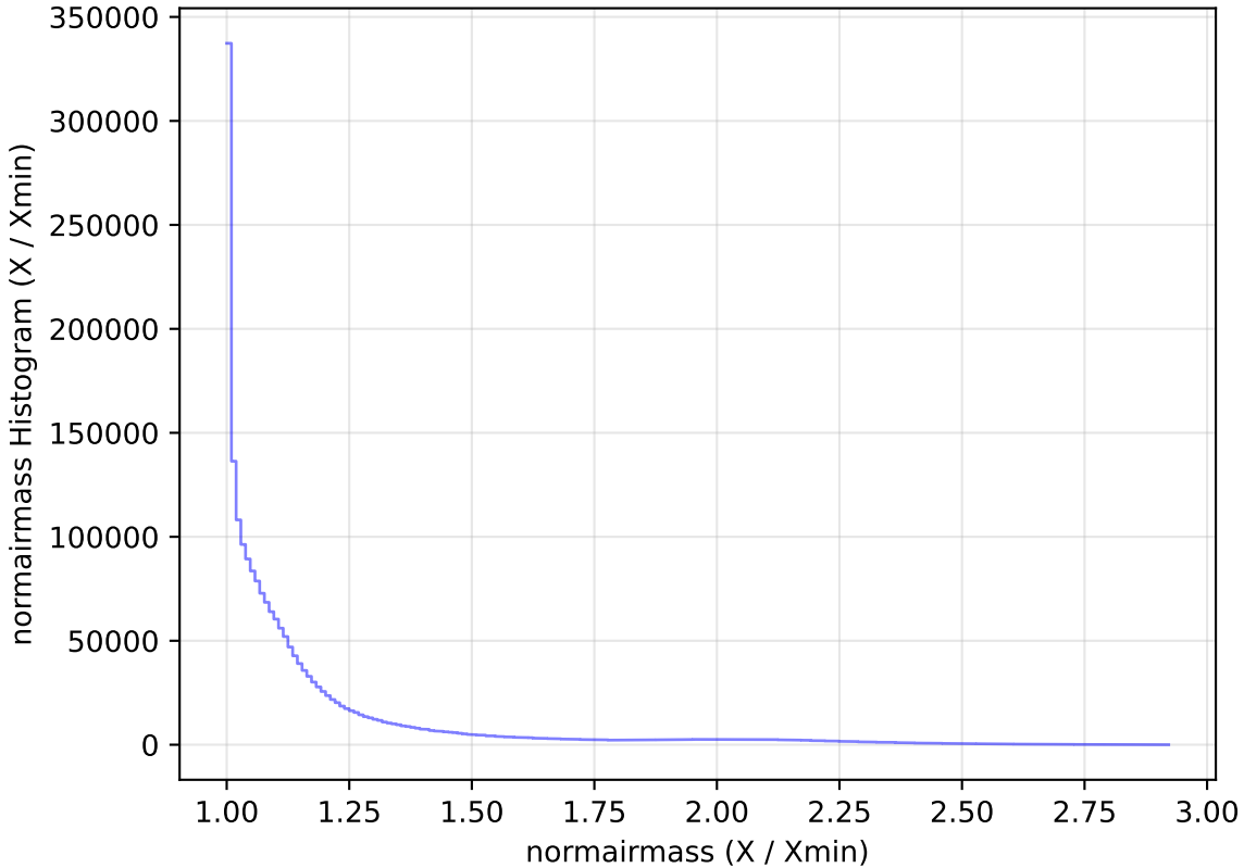
extra_ss_neo2_v3.4_10yrs WFD all bands: normairmass Histogram
