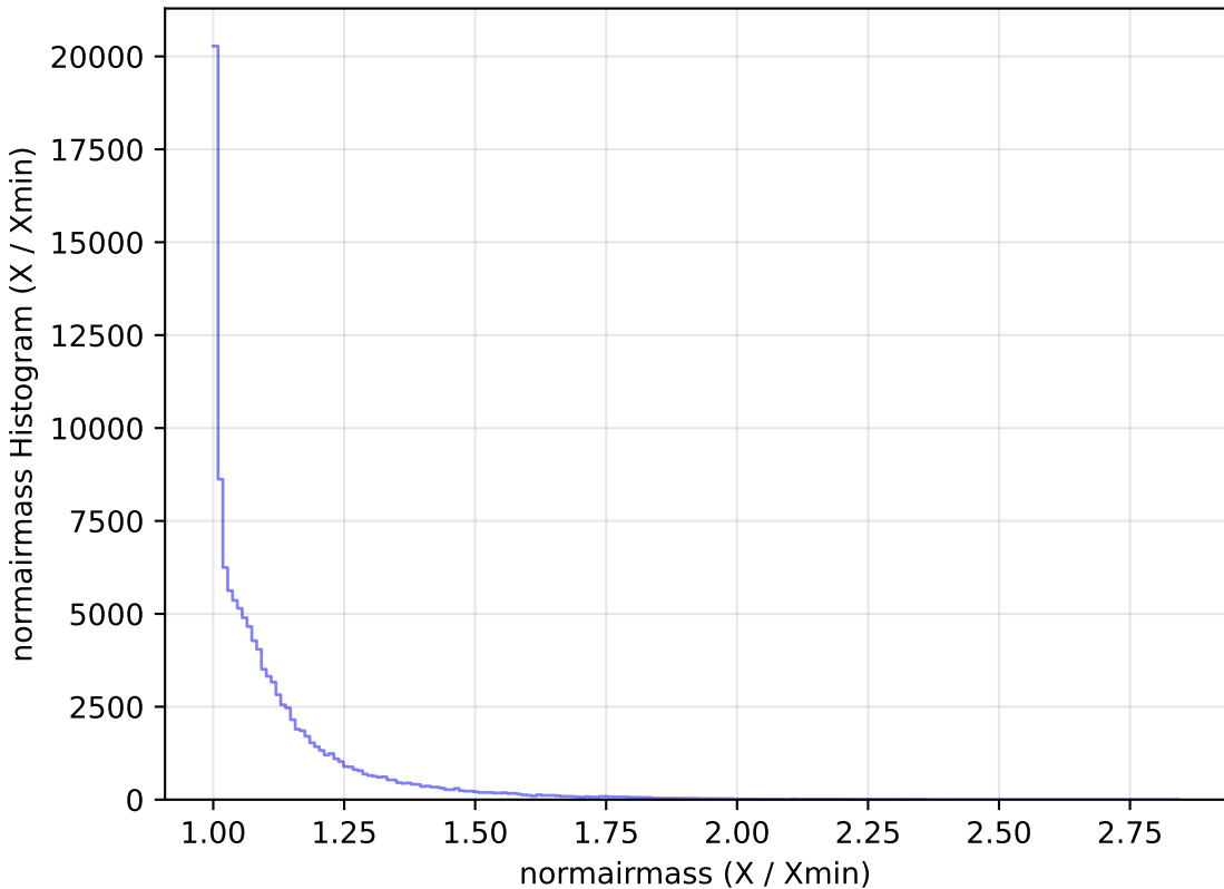
extra_ss_neo2_v3.4_10yrs All sky u band: normairmass Histogram
