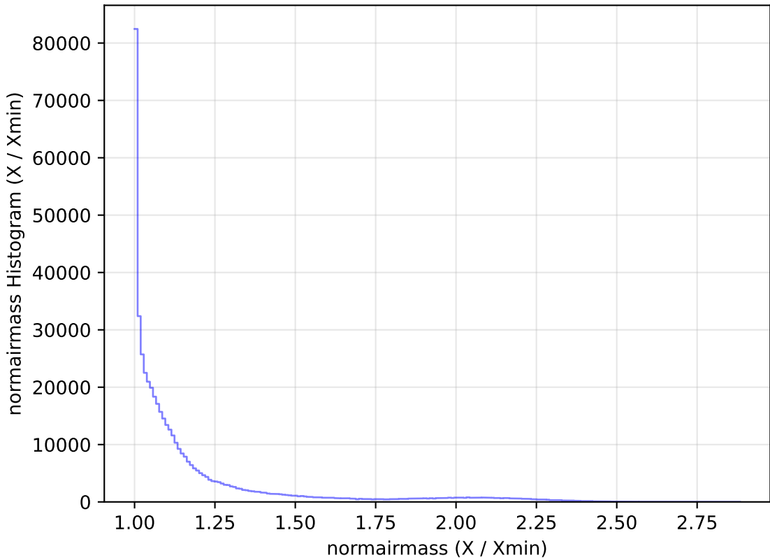
extra_ss_neo2_v3.4_10yrs All sky r band: normairmass Histogram
