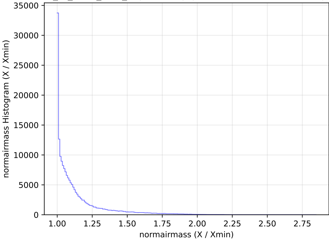
extra_ss_neo2_v3.4_10yrs All sky g band: normairmass Histogram
