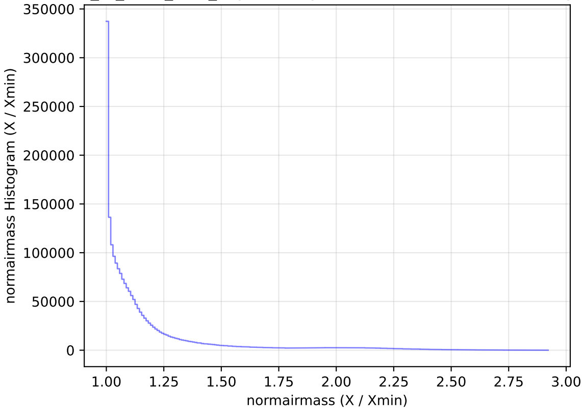
extra_ss_neo2_v3.4_10yrs All sky all bands: normairmass Histogram
