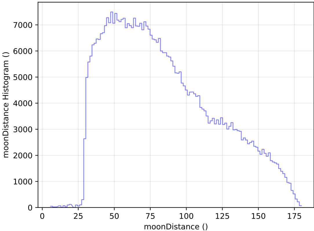
extra_ss_neo2_v3.4_10yrs WFD z band: moonDistance Histogram
