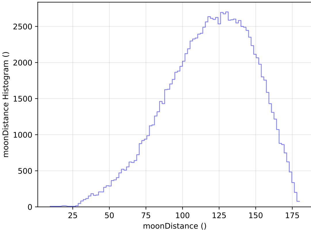
extra_ss_neo2_v3.4_10yrs WFD u band: moonDistance Histogram
