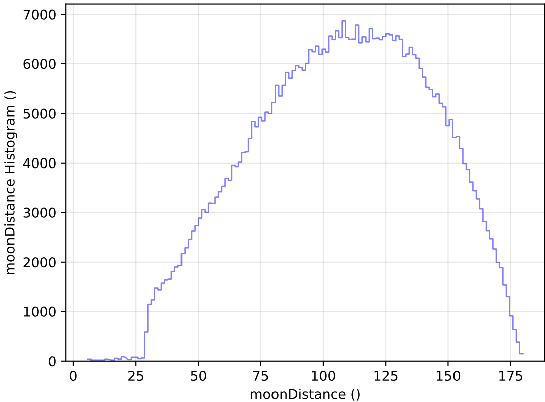
extra_ss_neo2_v3.4_10yrs WFD r band: moonDistance Histogram
