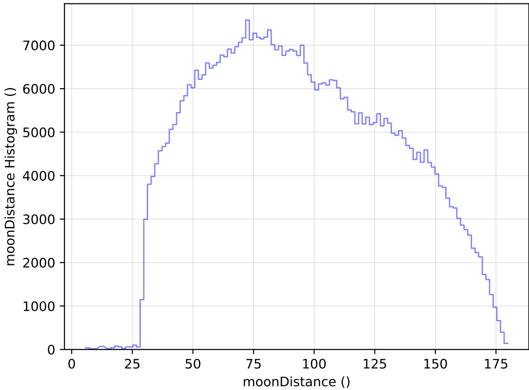
extra_ss_neo2_v3.4_10yrs WFD i band: moonDistance Histogram
