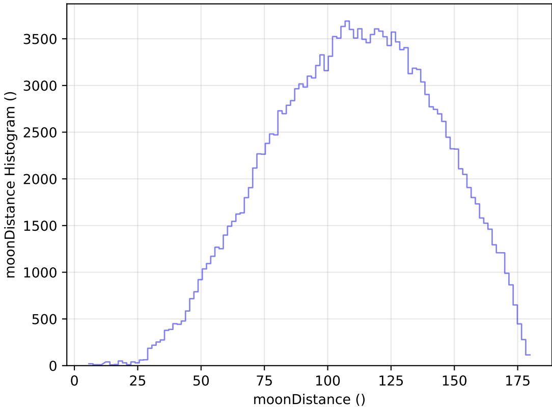
extra_ss_neo2_v3.4_10yrs WFD g band: moonDistance Histogram
