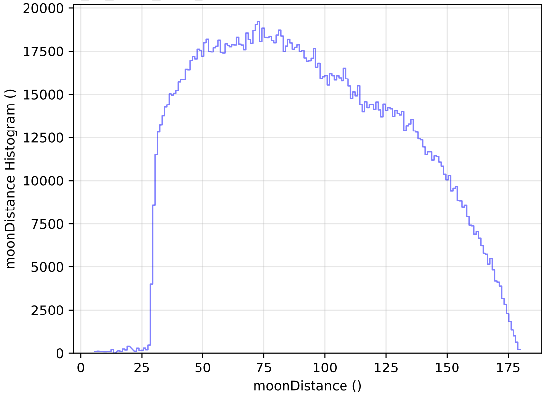
extra_ss_neo2_v3.4_10yrs WFD all bands: moonDistance Histogram
