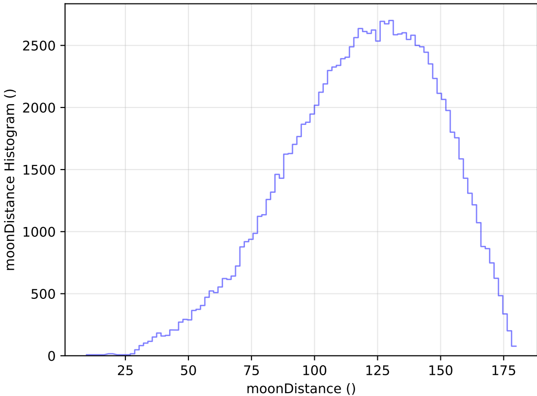
extra_ss_neo2_v3.4_10yrs All sky u band: moonDistance Histogram
