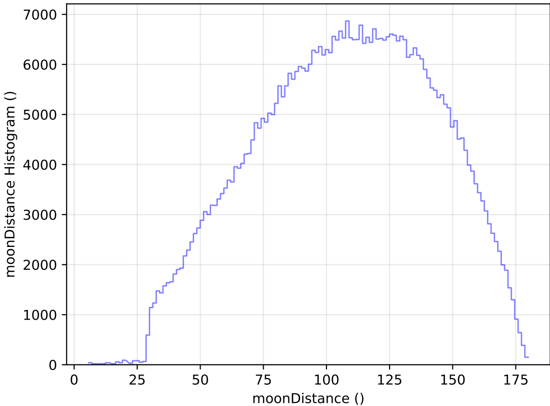
extra_ss_neo2_v3.4_10yrs All sky r band: moonDistance Histogram
